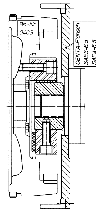
CENTA-H-30-1 KHD B/FL 912/913
